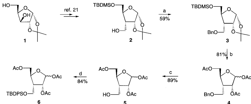
Scheme 1. Reagents: (a) BnBr, NaH, n -Bu 4 NI, DMF, 0°C. (b) i. 50% AcOH, 100°C; ii. Ac 2 O, pyridine. (c) Pd(OH) 2 , cyclohexene, EtOH, 80°C. (d) TBDPSCl, imidazole, DMF, rt.
