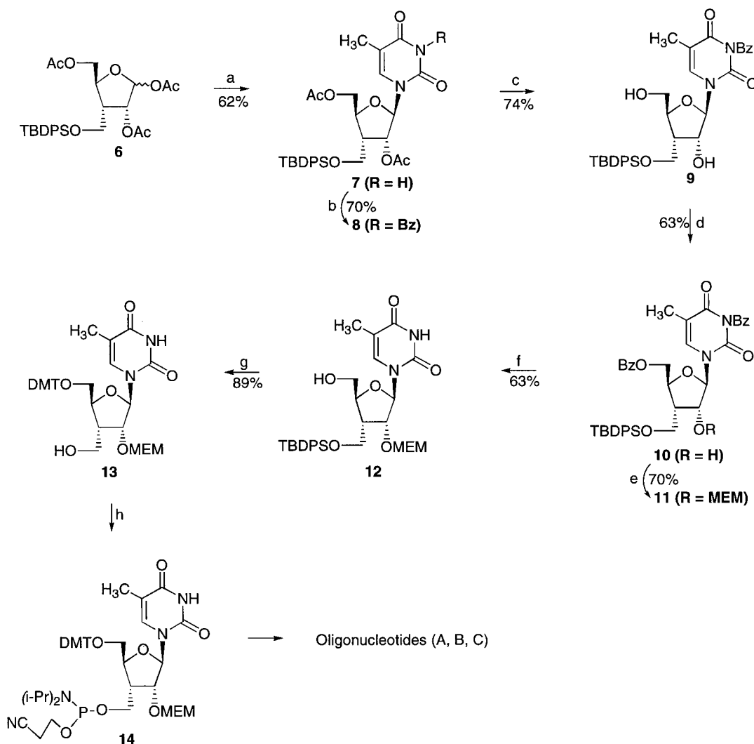
Scheme 2. Reagents: (a) Silylated thymine, TMSOTf, \text{CH}_2\text{Cl}_2 , rt to 50^\circ\text{C} . (b) BzCl, pyridine, 80^\circ\text{C} . (c) \text{K}_2\text{CO}_3 , MeOH, -5^\circ\text{C} . (d) BzCl, pyridine, -5^\circ\text{C} . (e) MEMCl, \text{CH}_2\text{Cl}_2 , i\text{-Pr}_2\text{NEt} . (f) \text{NH}_3 , MeOH, rt. (g) i. DMTCl, pyridine, rt; ii. n\text{-Bu}_4\text{NF} , THF, rt. (h) (i\text{-Pr})_2\text{NPCI}(\text{O})\text{CH}_2\text{CH}_2\text{CN} , i\text{-Pr}_2\text{NEt} , rt.
